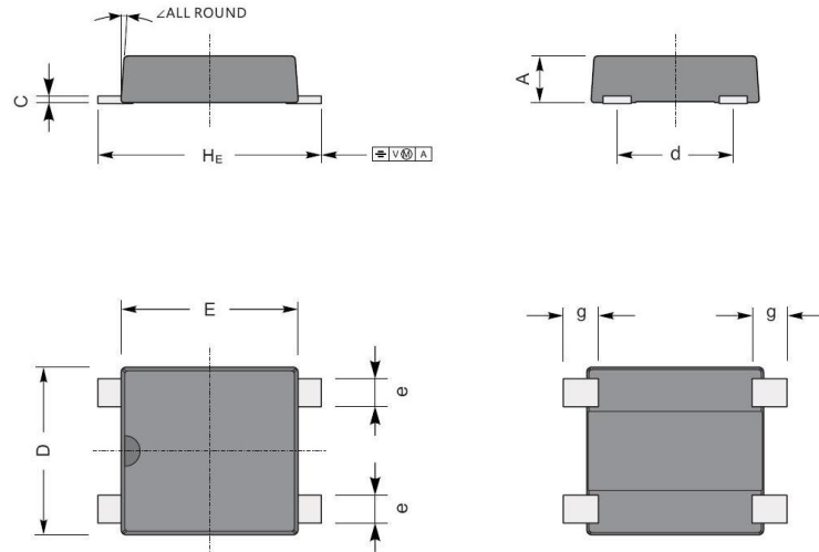
UMB mechanical data
